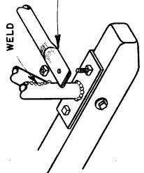
SKID CONNECTION DETAIL (STRUTS ARE REMOVED AFTER MOVING)
