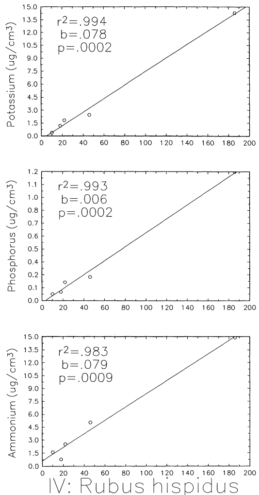
Fig. 2. Regression analysis of importance values and \text{NH}_4^+ -N, P, K, concentrations in soil with Rubus hispida . Calcium and magnesium show similar r^2 values, slopes and significance.
